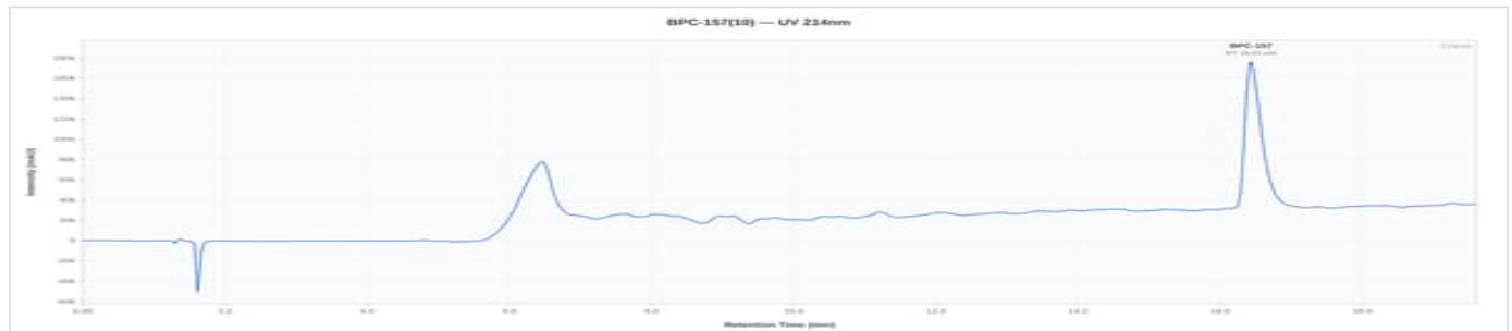
BPC-157 10mg - PRIME1026: UV Chromatogram
