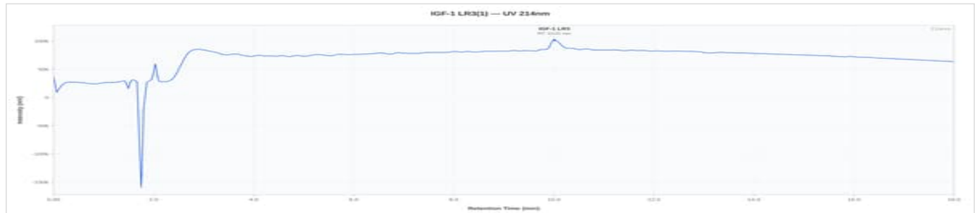
IGF-1 LR3 1 - PRIME1026: UV Chromatogram
