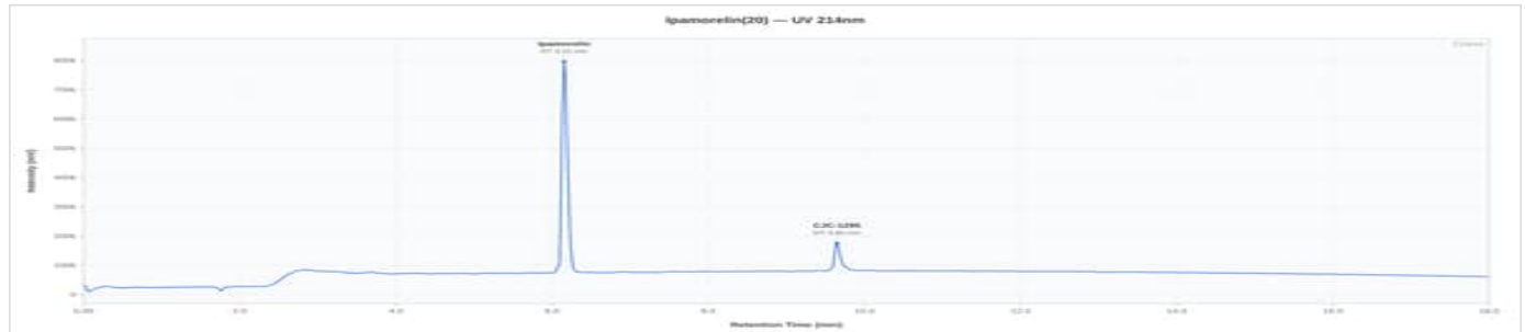
CJC-1295 no DAC + Ipamorelin 20 - PRIME1026: UV Chromatogram
