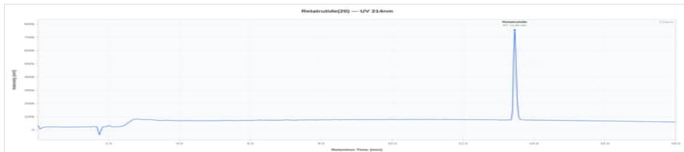
GLP-3 RT 20 - PRIME1026: UV Chromatogram
